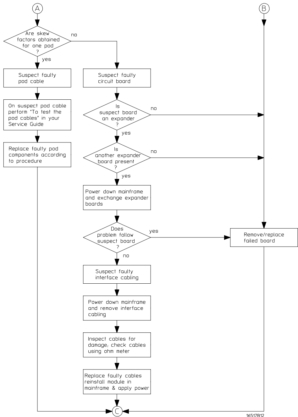
Troubleshooting Flowchart 2
